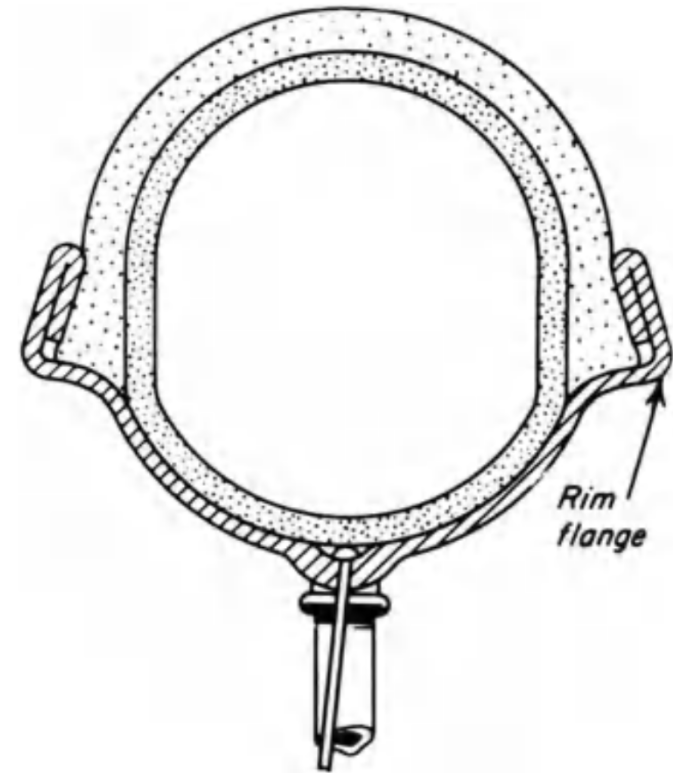
William Bartlett's rim and bead design of 1890.
