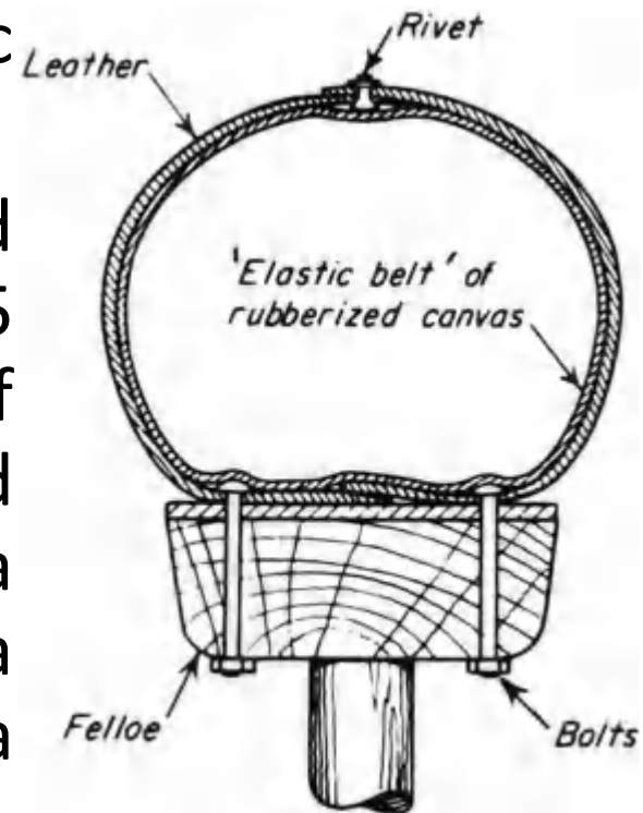
Thomson's original pneumatic tyre of 1845
