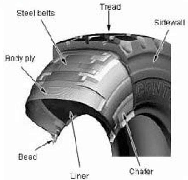
Radial Tyre
