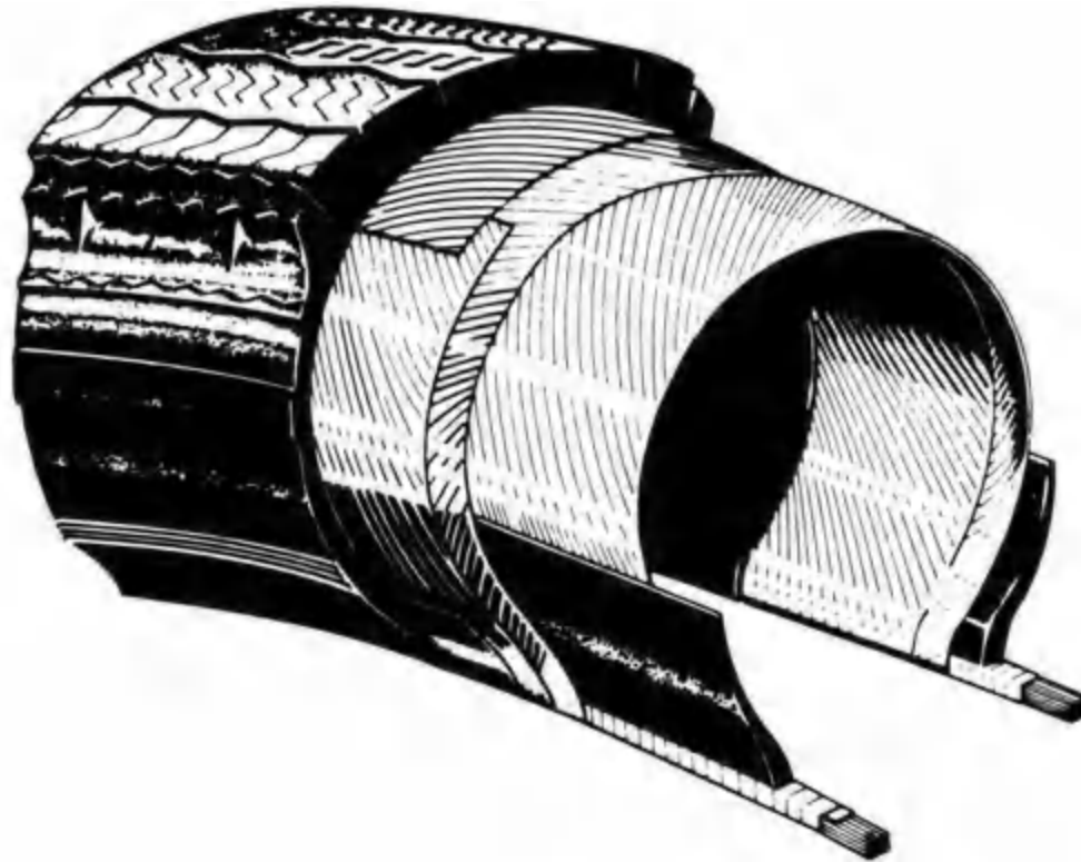
Internal construction of cross-ply tyre.
