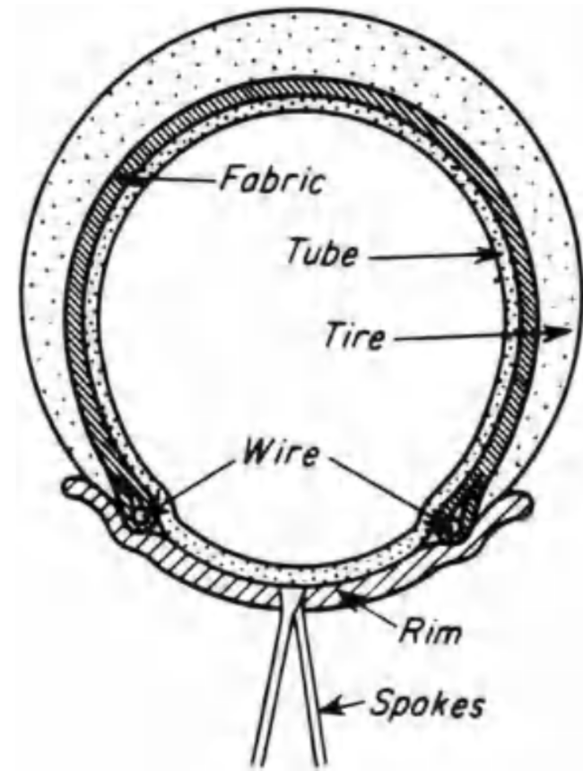
C. K. Welch's rim and bead design of 1890
